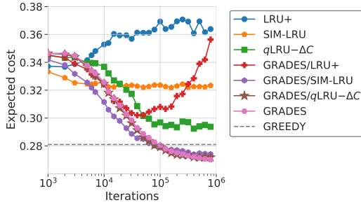
Fig. 4: Expected cost \mathcal{C}(\cdot) incurred by different policies under the trace Synthetic in Table I: LRU+, SIM-LRU, q\text{LRU-}\Delta C ( q = 10^{-2} ), GREEDY, and GRADES ( \eta = 0.64 , plain and grafted with p = 10^{-1} ). Cache size k = 313 .
