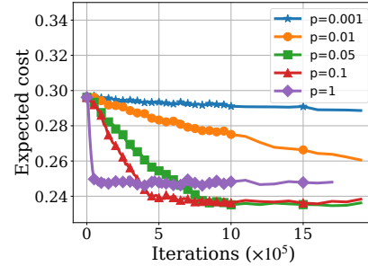
Fig. 6: Effect of grafting parameter p on the expected cost \mathcal{C}(\cdot) in a dynamic setting for GRADES/ q\text{LRU-}\Delta C ( \eta = 0.64 ). The cache is initialized to a stationary configuration as in Fig. 3. Now, only requests corresponding to region B from the synthetic trace are made. Cache size k = 313 .
