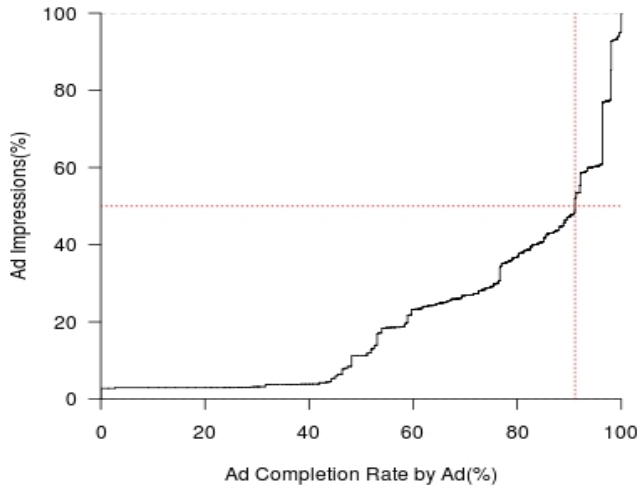
Figure 4: The percent of ad impressions y attributed to ads with ad completion rate smaller than x . 50% of the ad impressions are from ads with completion rate at most 91%.
