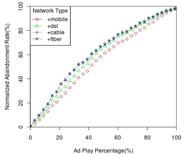
Figure 19: Normalized abandonment rates are roughly similar for the different connection types.
