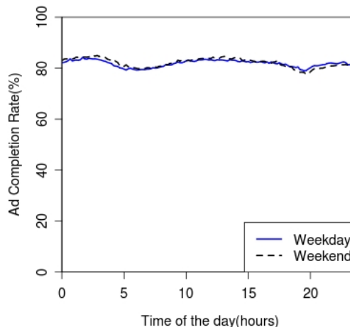
Figure 16: However, ad completion rates do not show major weekday/weekend or time-of-day variations.
