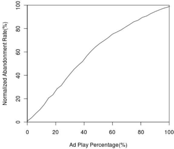
Figure 17: Normalized abandonment rate as a function of ad play percentage has a concave form. Of the viewers who eventually abandon the ad, about a third of the them have abandoned before the quarter-way mark and two-thirds of them have abandoned before the half-way mark.
