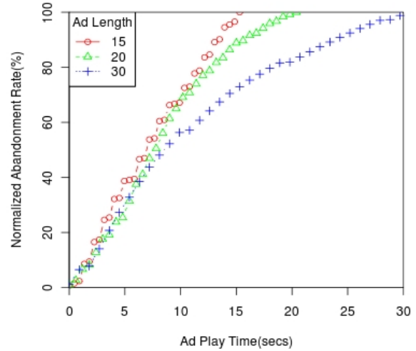
Figure 18: Normalized abandonment rate for different ad lengths.
