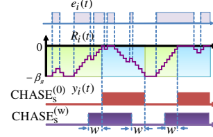
Figure 4: An example of e_i(t) , R_i(t) and the corresponding solution obtained by CHASE s (w) for EP i .
