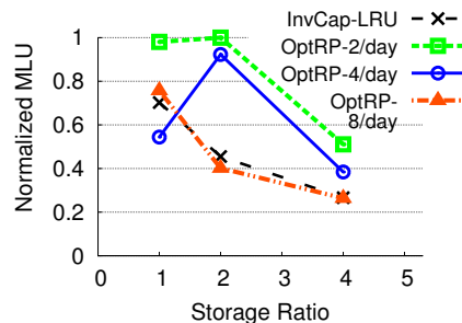
Figure 12: [Entertainment, US-ISP] OptRP does not outperform InvCap-LRU despite engineering 8 times a day.
