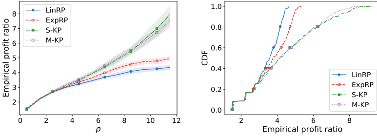
Fig. 4. The impact of different knapsack capacities on different algorithms. Different capacities are represented by parameter \rho = \theta \in [=] \vartheta \in [ < ] w \theta \cdot \vartheta / C , e.g., \rho = 10 represents the case that the aggregate item size is 10 times than that of the aggregate capacity of knapsack, i.e., demand is roughly 10 times the available resource.
