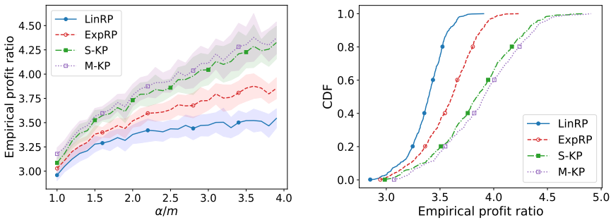
Fig. 3. The impact of \alpha (captures heterogeneity on the capacity of dimensions) on different algorithms. Parameter \alpha = \frac{1}{g} C_g / \min_g C_g is the ratio between the aggregate capacity of knapsack and the minimum single-dimension capacity, e.g., \alpha/m = 1 represent the case that dimensions have the same capacity.
