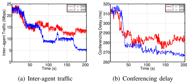
Fig. 4. Evolution of traffic and delay over time (200 seconds) by executing Alg. 1 with different \beta s and Nrst for initial assignment
