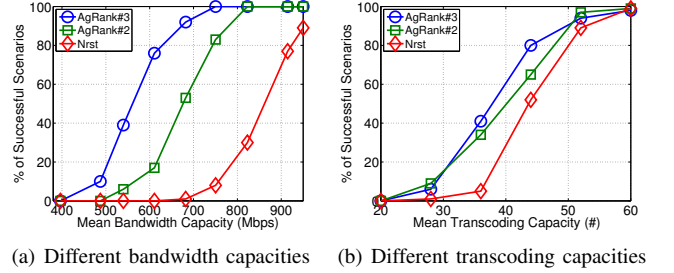
Fig. 9. Comparison of AgRank and Nrst
