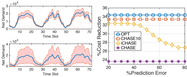
Figure 5: A sample illustration of net electricity demand as a function of interval prediction with 20% (top) and 80% (bottom) of the values
